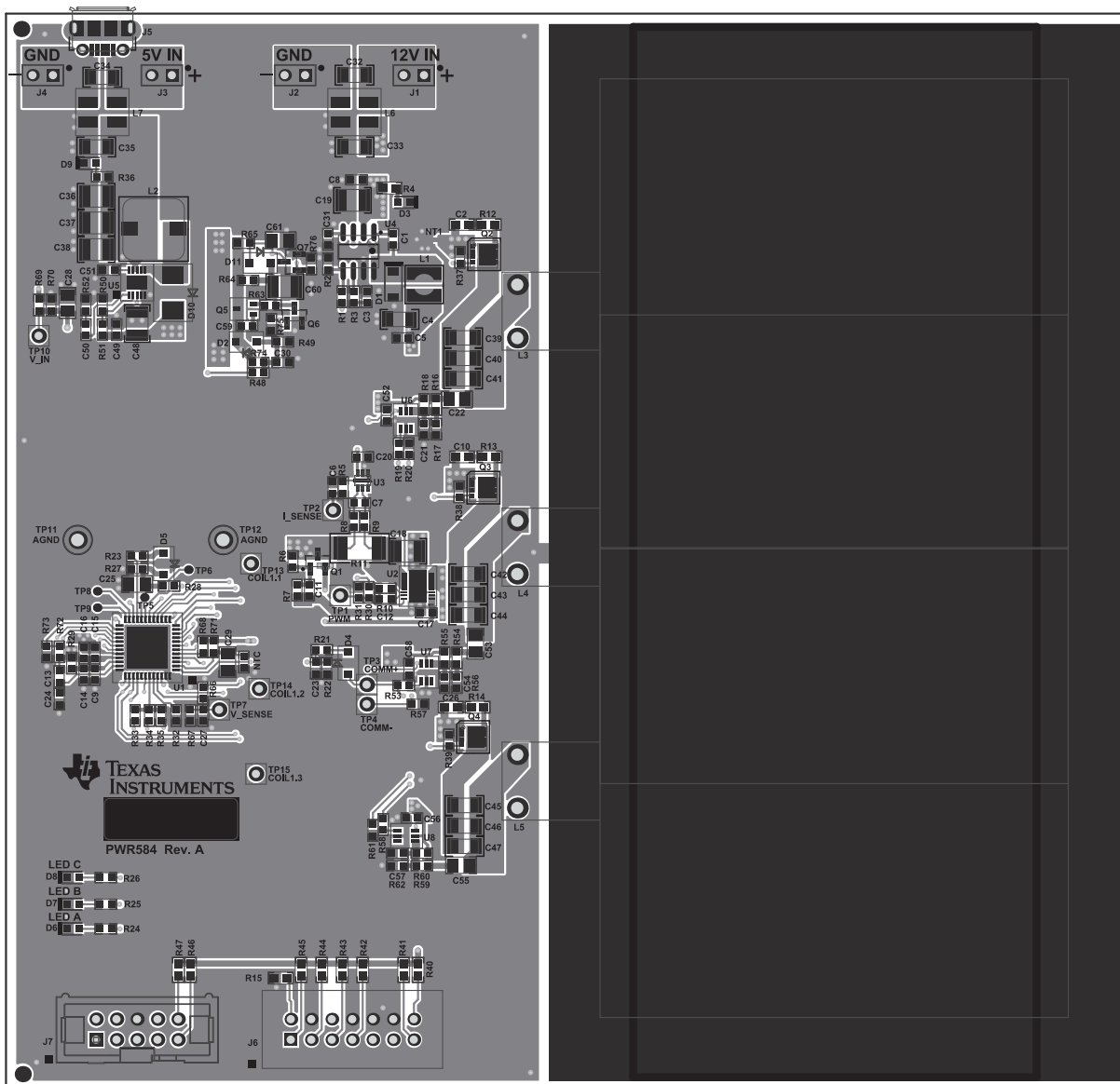
Figure 7. Top Layer
