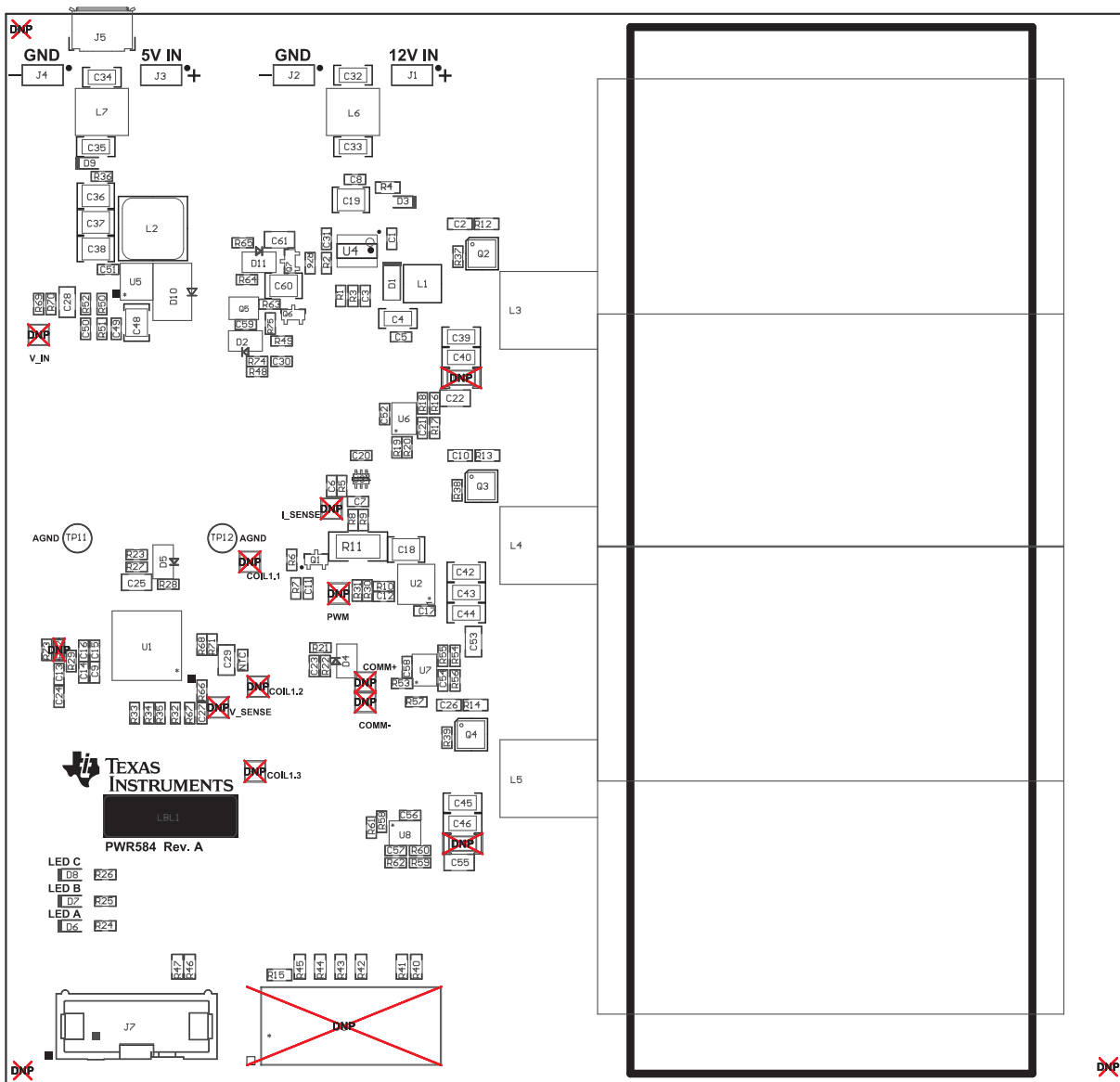
Figure 5. Assembly Top
