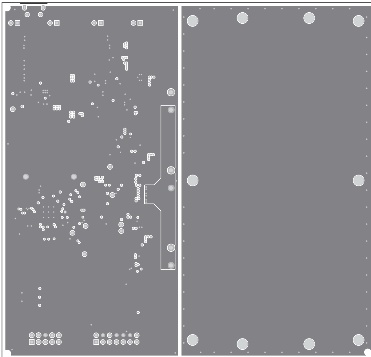
Figure 8. Layer 2
