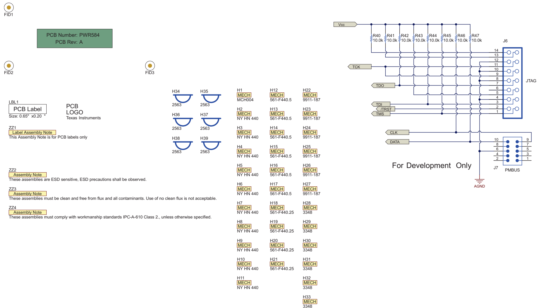
Figure 2. bq500412EVM-584 Schematic (2 of 2)
