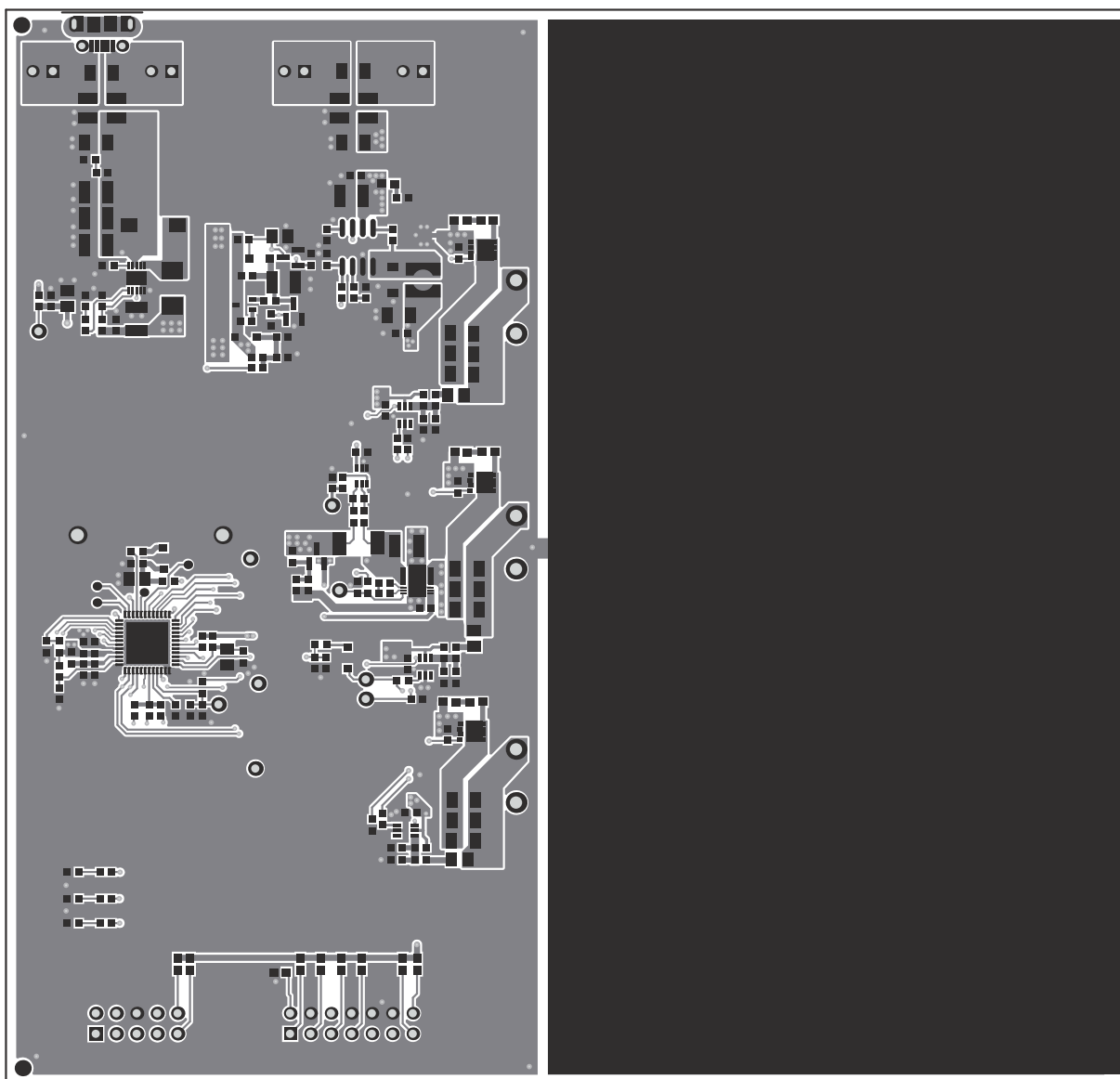
Figure 6. Top Silk
