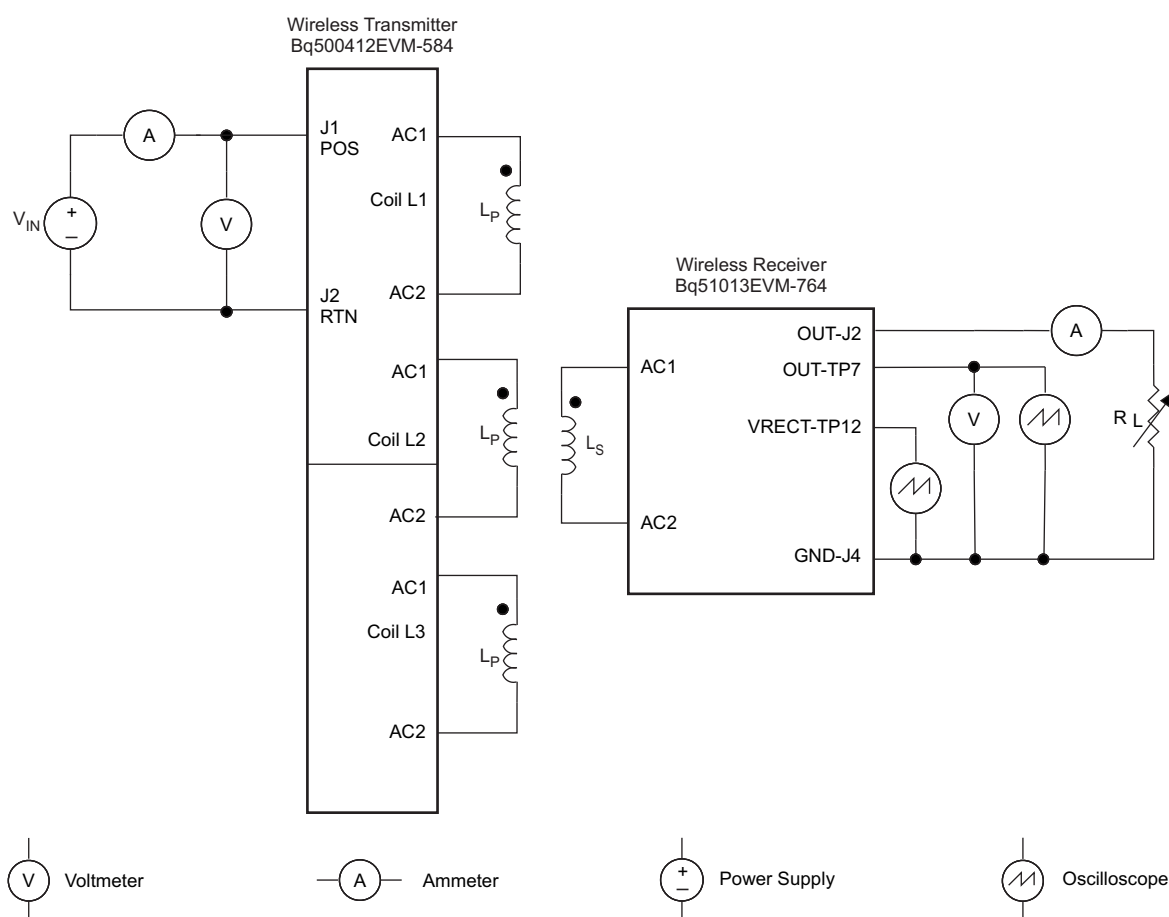
Figure 3. Equipment Setup
